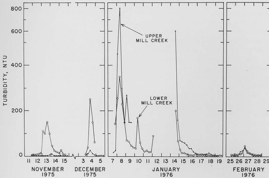
Figure 3. Stream turbidities in Mill Creek during periods of high runoff.
