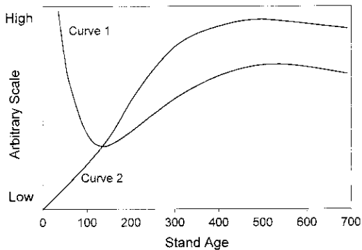
Figure 1. Idealized changes in ecosystems attributes during succession in Douglas-fir forests. (See Table 2 for description of curves, adapted from Spies and Franklin 1988.)
