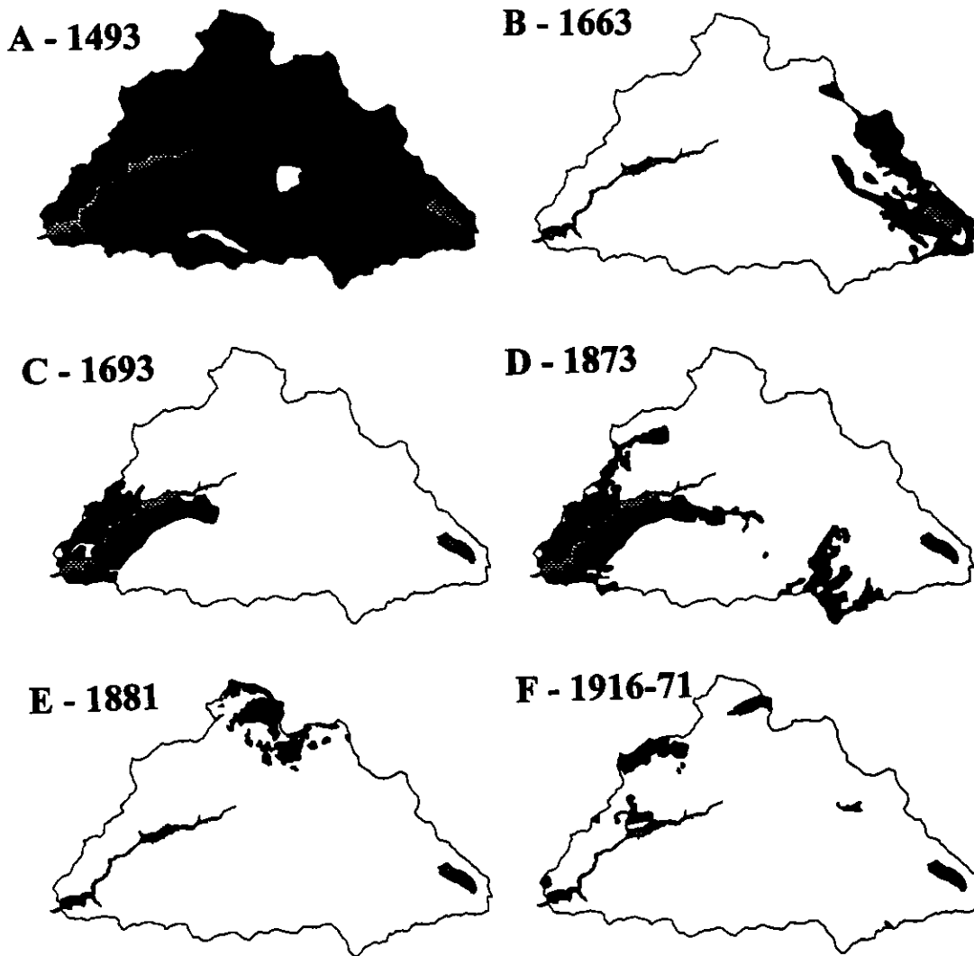
Figure 3. Reconstructed extent of historic fires in the Bull Run watershed. A. 1493 A.D. fire. The ca. 1243 A.D. fire is shown as two small white polygons. B. 1663 A.D. fire appears to have entered the watershed from the east. C. 1693 A.D. fire is in the lower western portion of the watershed. D. 1873 A.D. fire covers much of the same area as the 1693 fire plus a separate area on the southern edge of the watershed. E. 1881 A.D. fire is a patchy fire at the northern edge of the watershed. F. Twentieth century fires (1916 A.D. through 1971 A.D.) are small and scattered.
