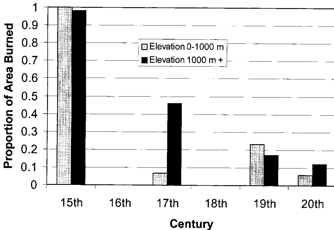
Figure 4. The proportion of the watershed burned by century by elevation zone. There is a decreasing proportion over time, and no apparent trend by elevation zone.
