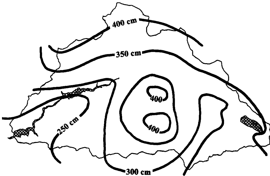
Figure 2. Annual precipitation within the Bull Run (data from City of Portland, Oregon, Bureau of Water Works).
