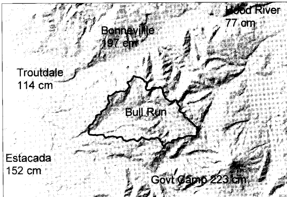
Figure 1. Location of Bull Run watershed in northwest Oregon. The Bull Run is located just south of the Columbia River, flowing in this figure from Hood River west to Bonneville and Troutdale. Annual precipitation for neighboring weather stations shown (Website http://www.wrcc.dri.edu/summary/climsmor.html ). Mount Hood is the obvious peak in the southeast corner of the frame. Data for figure supplied by Diana Sinton.
