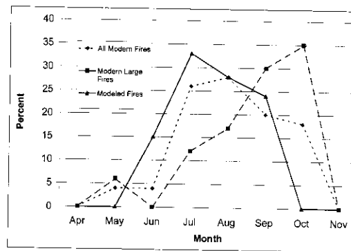
Figure 5. Proportional seasonal distribution of twentieth century fires. Modern fires are those within the watershed, and large modern fires are those exceeding 0.1 ha in size. Modeled fires are for the Wind River area (just north of Bonneville in Figure 1) and are for fires exceeding 1 ha in size.
