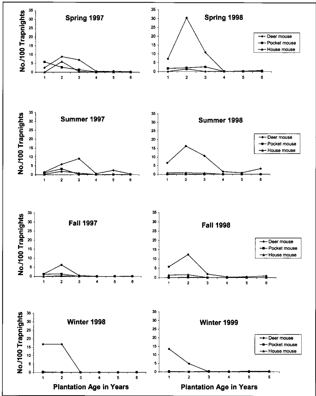
Figure 1. Change in rodent species abundance (number individuals per 100 trap nights) relative to stand age, spring 1997 through winter 1999.
