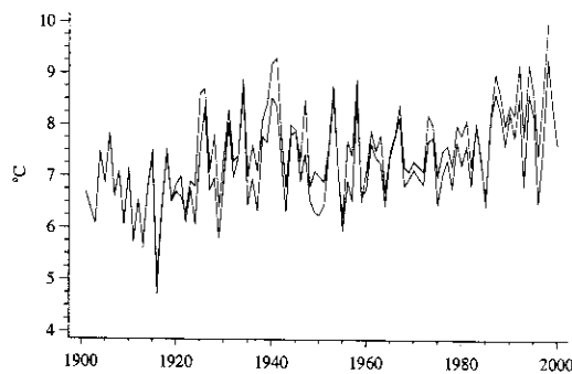
Figure 3. Comparison of annual mean temperature at Porthill, Idaho (lower), period of record 1901-2000 from the USHCN dataset, and Creston, British Columbia (upper), period of record 1913-1998 from the HCCD dataset. The two stations are about 10 km apart and both records have been adjusted to remove various time-dependent biases.
