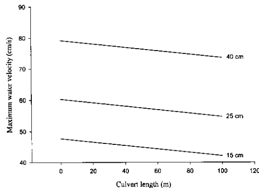
Figure 2. Maximum water velocities that will allow bull trout of three sizes to pass culverts of various lengths in 11° to 15°C water. The lines were determined as follows: maximum water velocity within a culvert equals the highest speed a fish can maintain for 30 min ( U_{crit30} ) minus the minimum ground speed required to pass the culvert in 30 min (culvert length/1,800 s). The U_{crit30} values were calculated by substituting length values into the appropriate equation from Figure 1.
