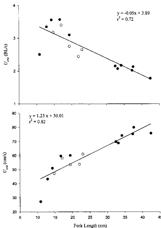
Figure 1. Linear regressions of U_{crit} (top panel = BL/s; bottom panel = cm/s) as a function of length for eleven fish swum at 11°C (black circles) and five fish at 15°C (open circles).
